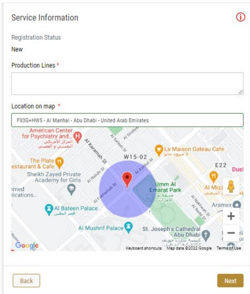
Figure 20 – User Data
